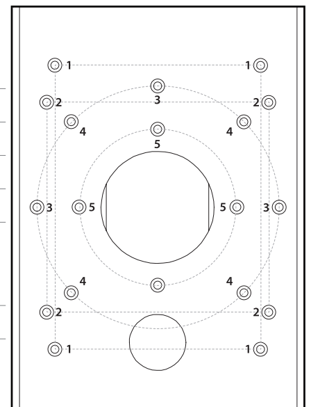
Pole mount front view
